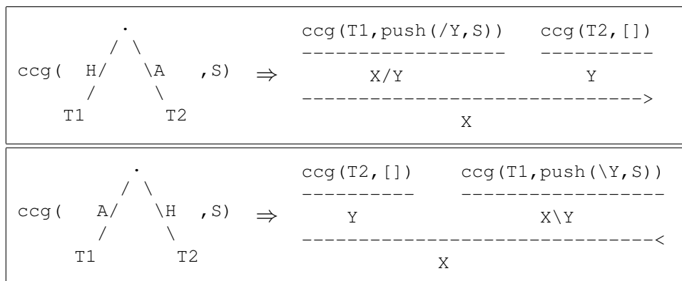
Figure 7: The argument case for translating binary trees to CCG.
