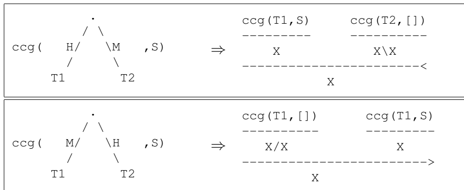
Figure 6: The modifier case for translating binary trees to CCG.
